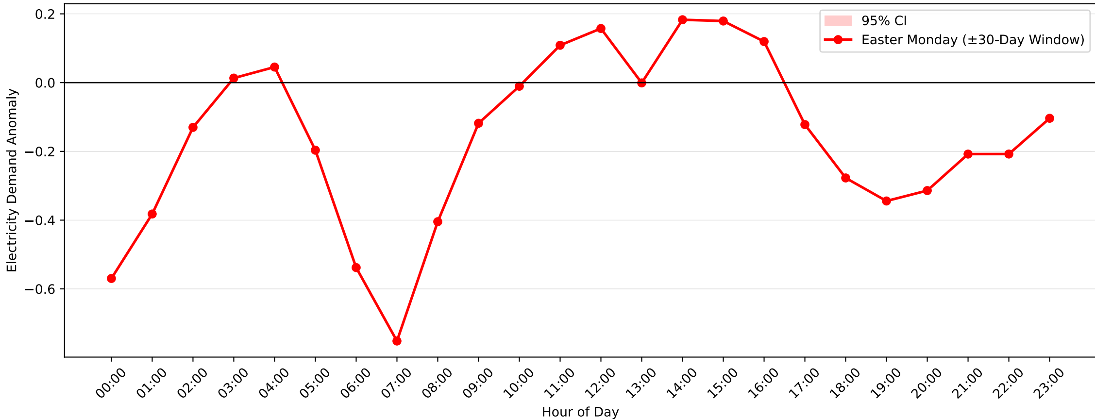
Jesmond Demand Anomaly: Easter Monday (2010-2011, \pm 30 -Day Window)
